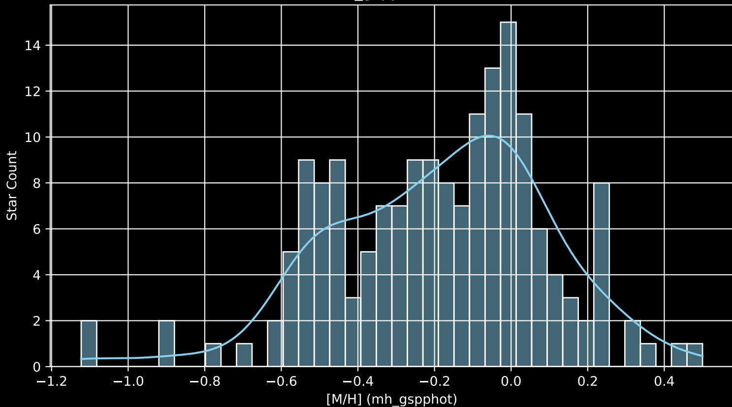
APOGEE DR17 Field: [178+24_MGA [M/H] (mh_gspphot) (n= 172)
