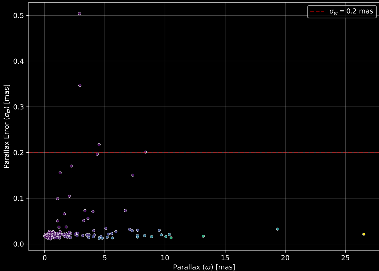
APOGEE DR17 Field: [178+24_MGA] Parallax Quality (n= 175)
