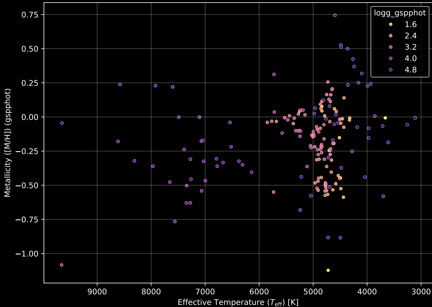
APOGEE DR17 Field: [178+24_MGA] Stellar Population Parameters (n= 175)
