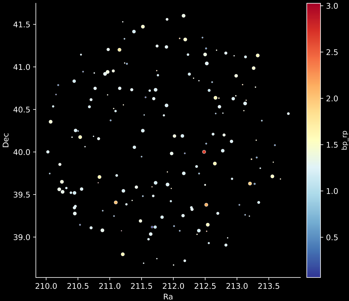
APOGEE DR17 Field: [178+24_MGA] Stars: 175
