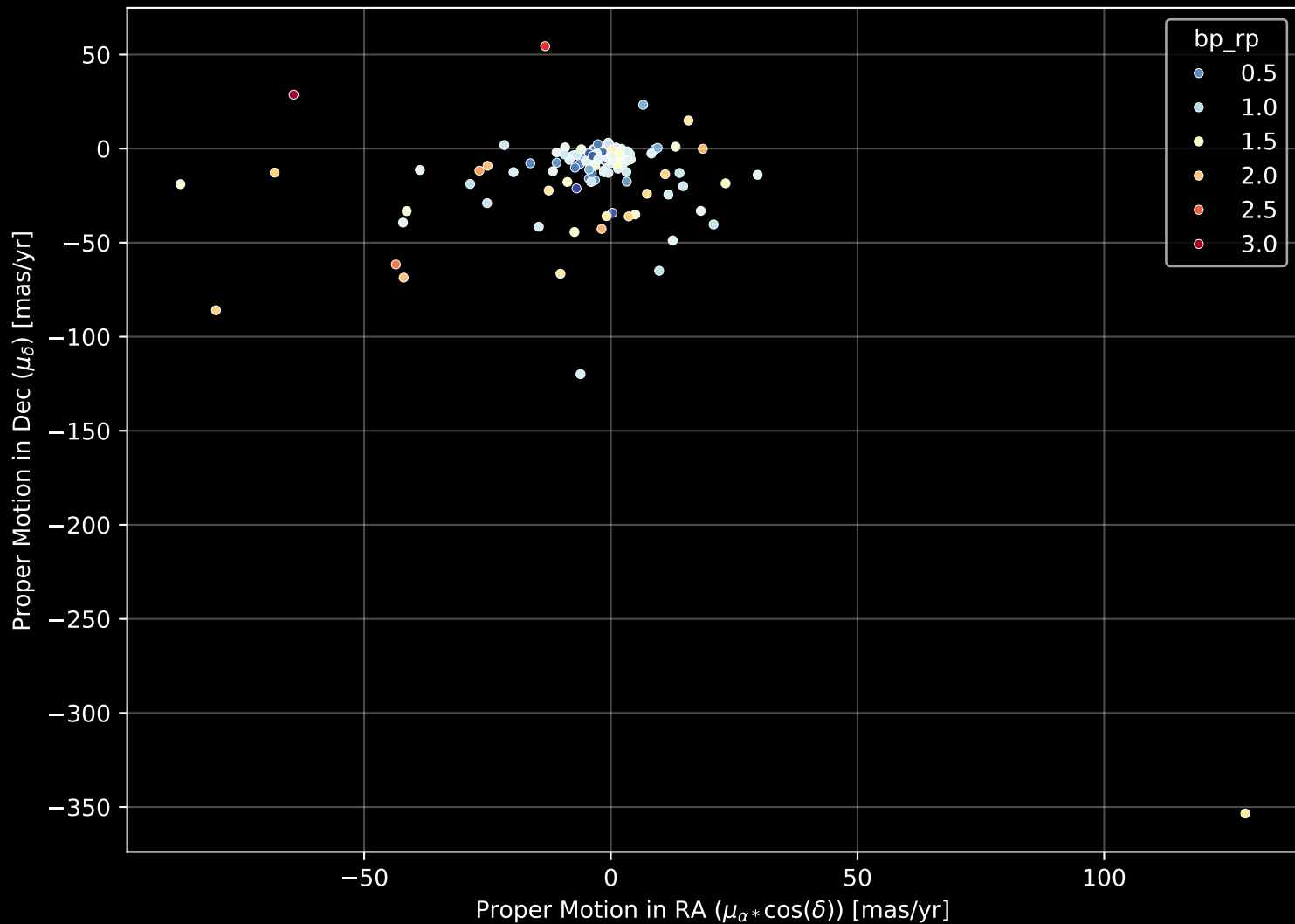
APOGEE DR17 Field: [178+24_MGA] Proper Motion Diagram (n= 175)
