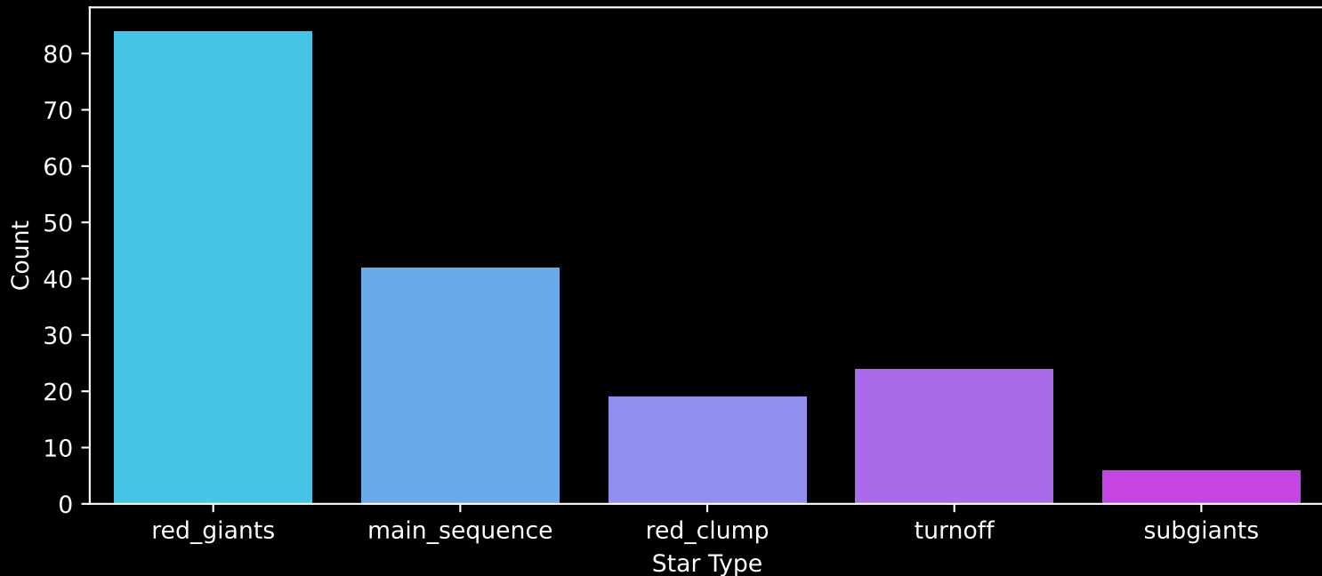
APOGEE DR17 Field: [178+24_MGA] Count plot of Star Type
