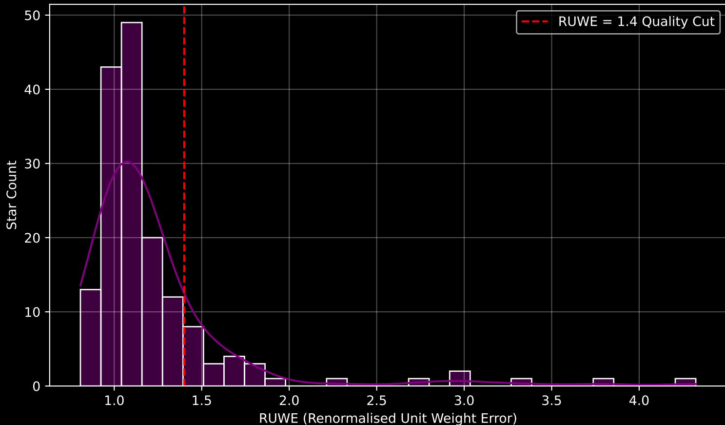
GAPOGEE DR17 Field [178+24_MGA] RUWE Distribution (n= 163)
